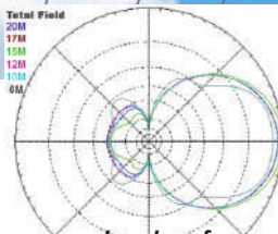
Gives monoband performance, no sidelobes.
